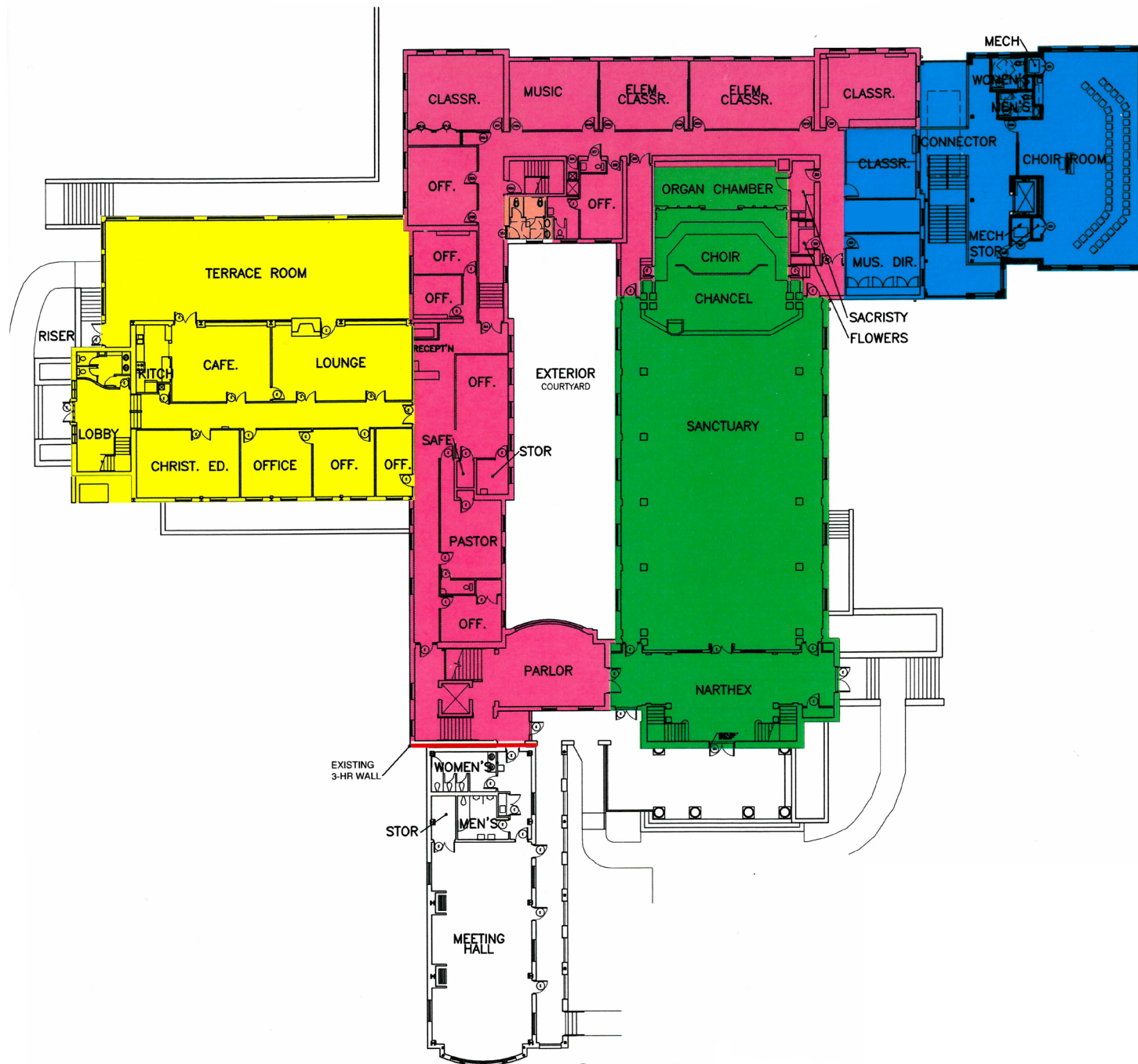
2 UPPER LEVEL SCALE: 1/16" = 1'-0"
